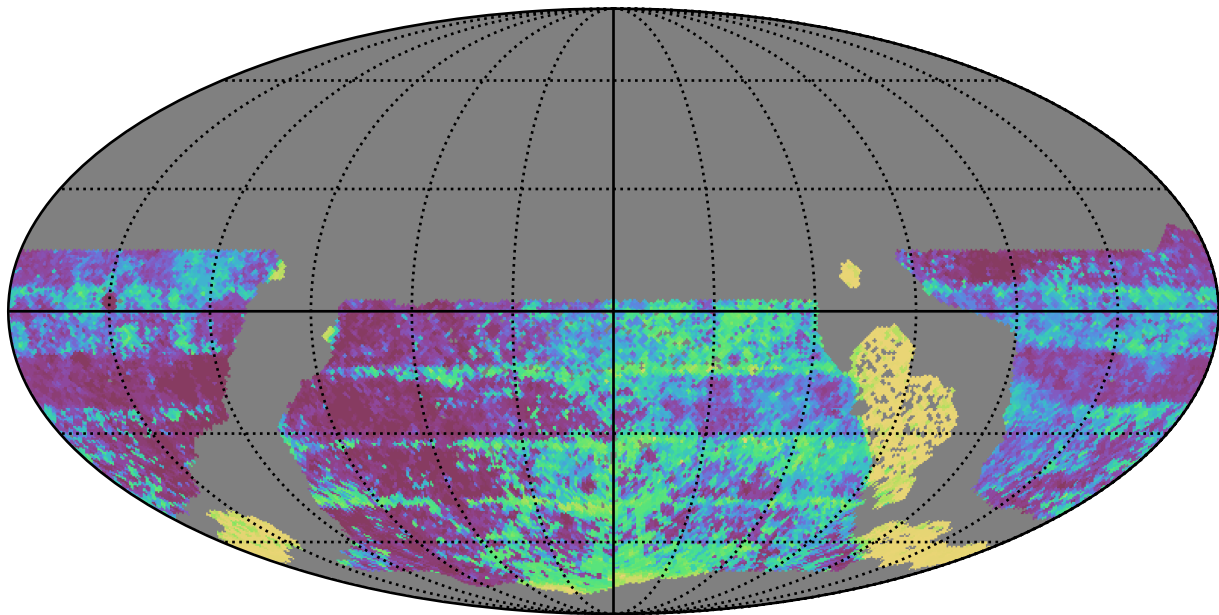
ddf_acor_sf20_lsf40_lsr50_v3.4_10yrs WFD y band: Median Inter-Night Gap
