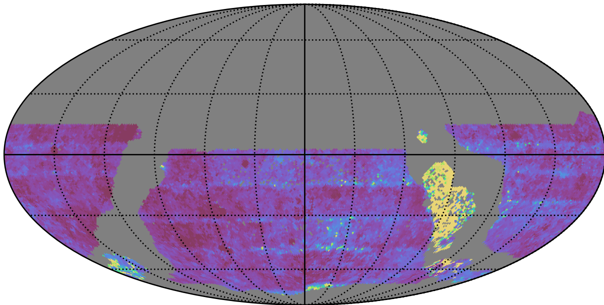
ddf_acor_sf20_lsf40_lsr50_v3.4_10yrs WFD u band: Median Inter-Night Gap
