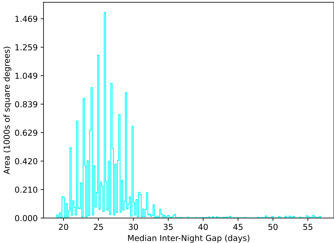
ddf_acor_sf20_lsf40_lsr50_v3.4_10yrs WFD u band: Median Inter-Night Gap
