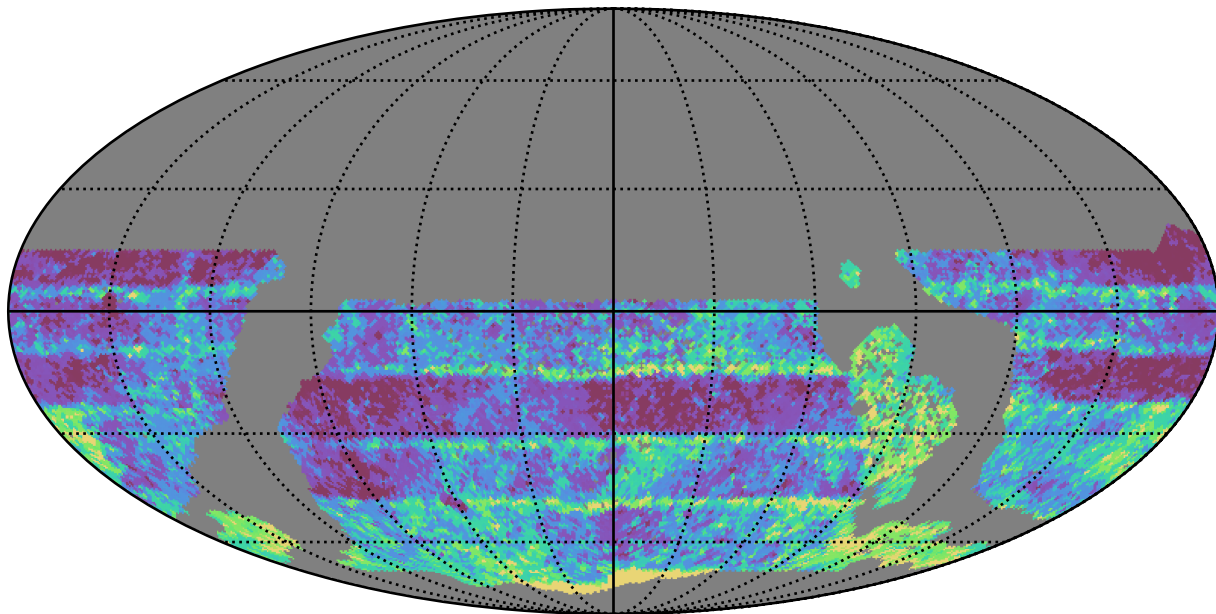
ddf_acor_sf20_lsf40_lsr50_v3.4_10yrs WFD r band: Median Inter-Night Gap
