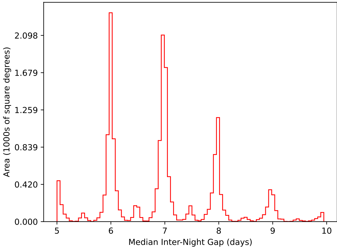
ddf_acor_sf20_lsf40_lsr50_v3.4_10yrs WFD i band: Median Inter-Night Gap
