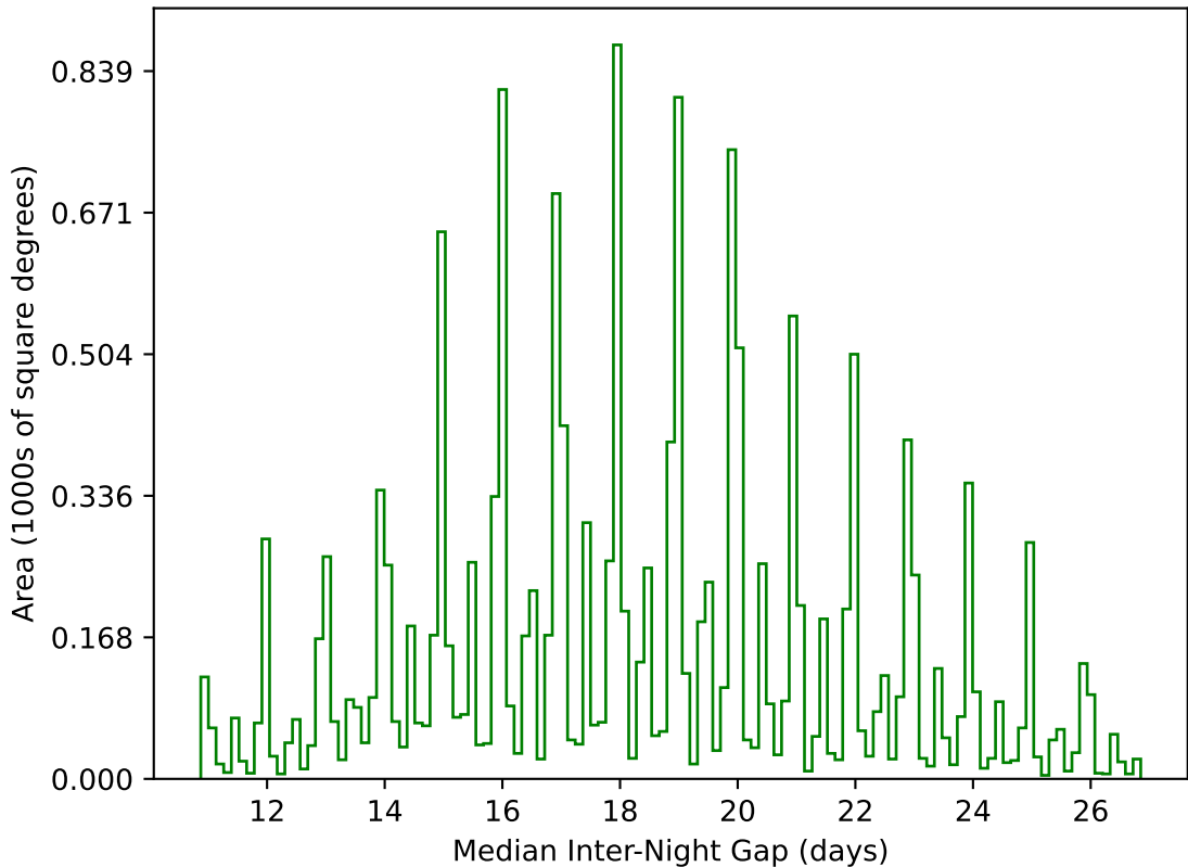
ddf_acor_sf20_lsf40_lsr50_v3.4_10yrs WFD g band: Median Inter-Night Gap
