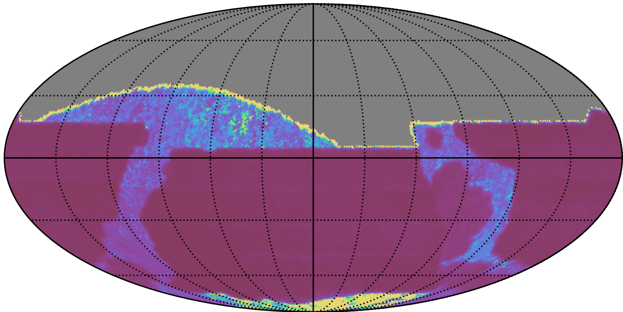
ddf_acor_sf20_lsf40_lsr50_v3.4_10yrs All sky z band: Median Inter-Night Gap
