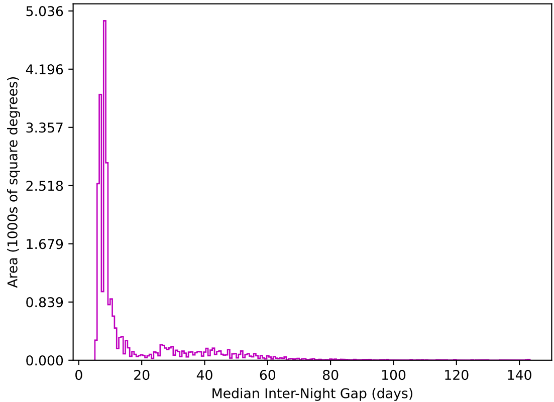
ddf_acor_sf20_lsf40_lsr50_v3.4_10yrs All sky z band: Median Inter-Night Gap
