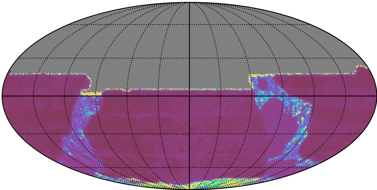
ddf_acor_sf20_lsf40_lsr50_v3.4_10yrs All sky y band: Median Inter-Night Gap
