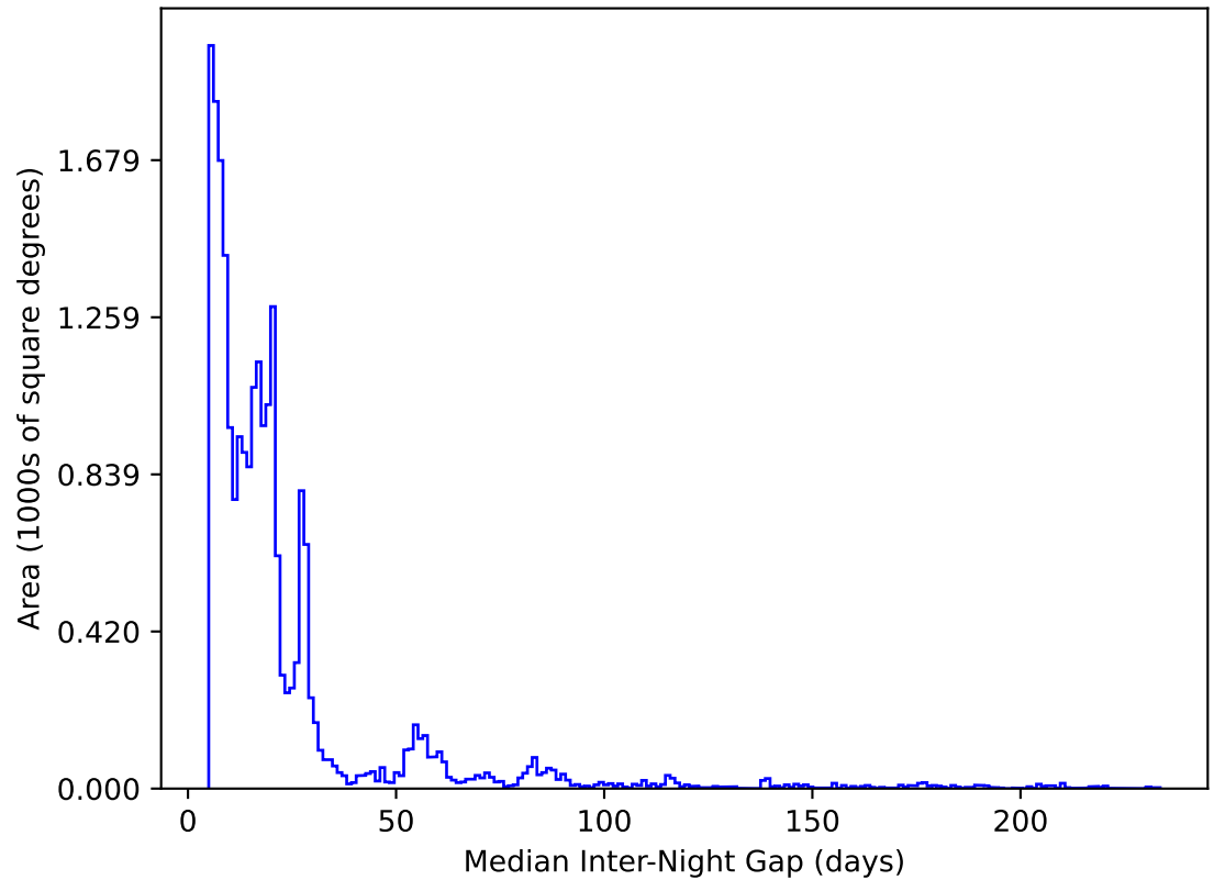
ddf_acor_sf20_lsf40_lsr50_v3.4_10yrs All sky y band: Median Inter-Night Gap
