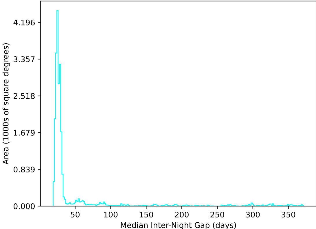
ddf_acor_sf20_lsf40_lsr50_v3.4_10yrs All sky u band: Median Inter-Night Gap
