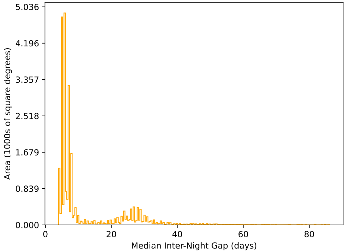
ddf_acor_sf20_lsf40_lsr50_v3.4_10yrs All sky r band: Median Inter-Night Gap
