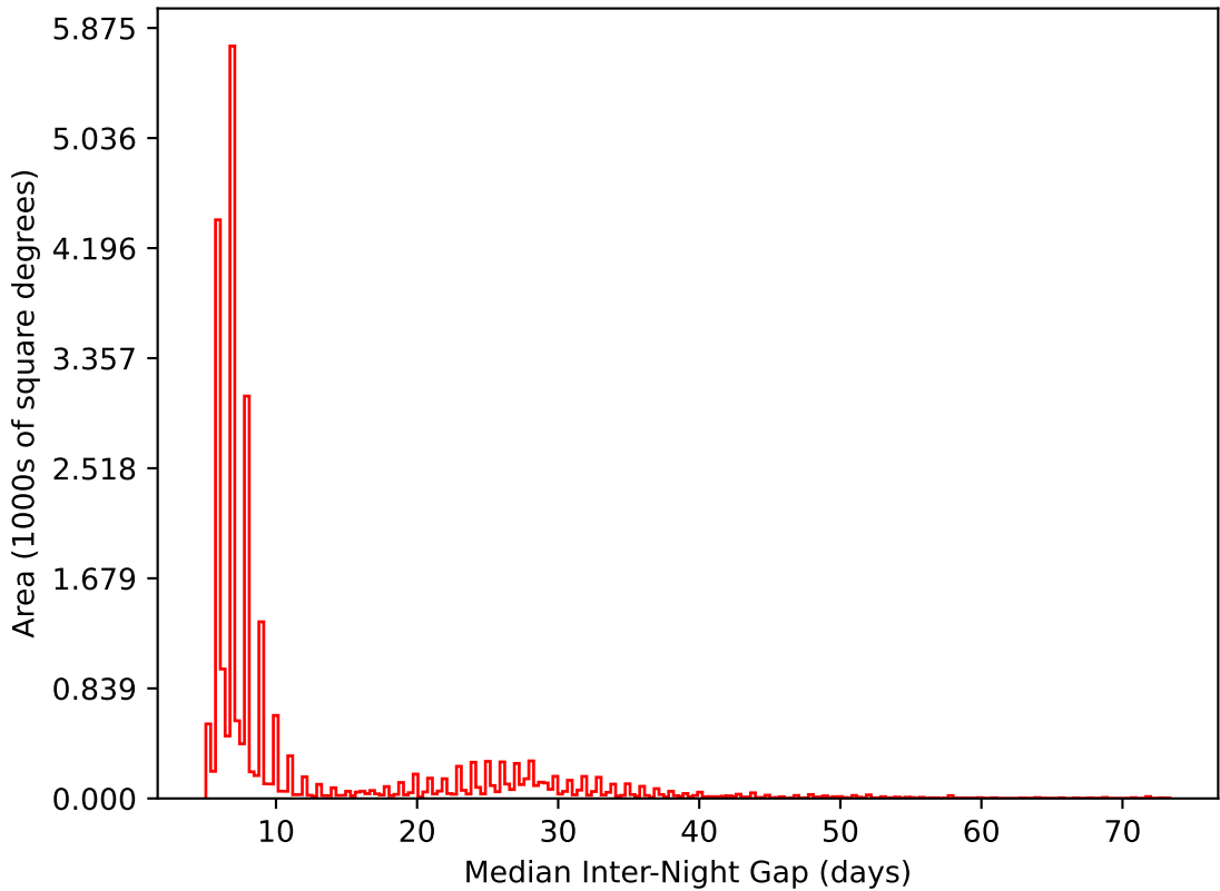
ddf_acor_sf20_lsf40_lsr50_v3.4_10yrs All sky i band: Median Inter-Night Gap
