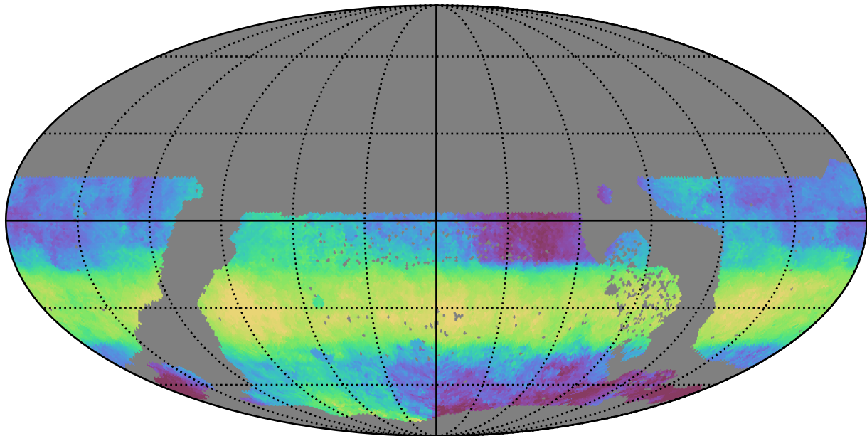
ddf_acor_sf20_lsf40_lsr50_v3.4_10yrs WFD z band: Median HA
