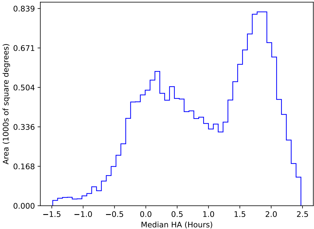
ddf_acor_sf20_lsf40_lsr50_v3.4_10yrs WFD u band: Median HA
