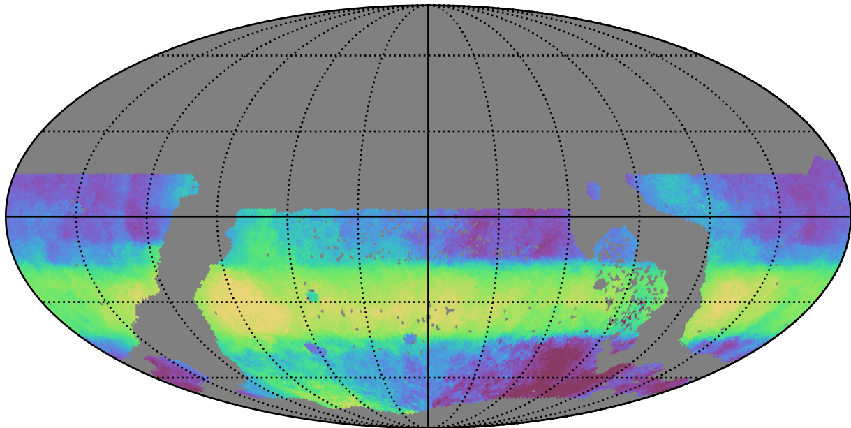
ddf_acor_sf20_lsf40_lsr50_v3.4_10yrs WFD r band: Median HA
