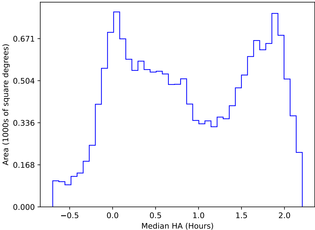
ddf_acor_sf20_lsf40_lsr50_v3.4_10yrs WFD r band: Median HA
