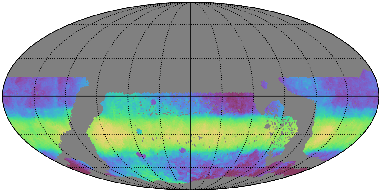
ddf_acor_sf20_lsf40_lsr50_v3.4_10yrs WFD i band: Median HA
