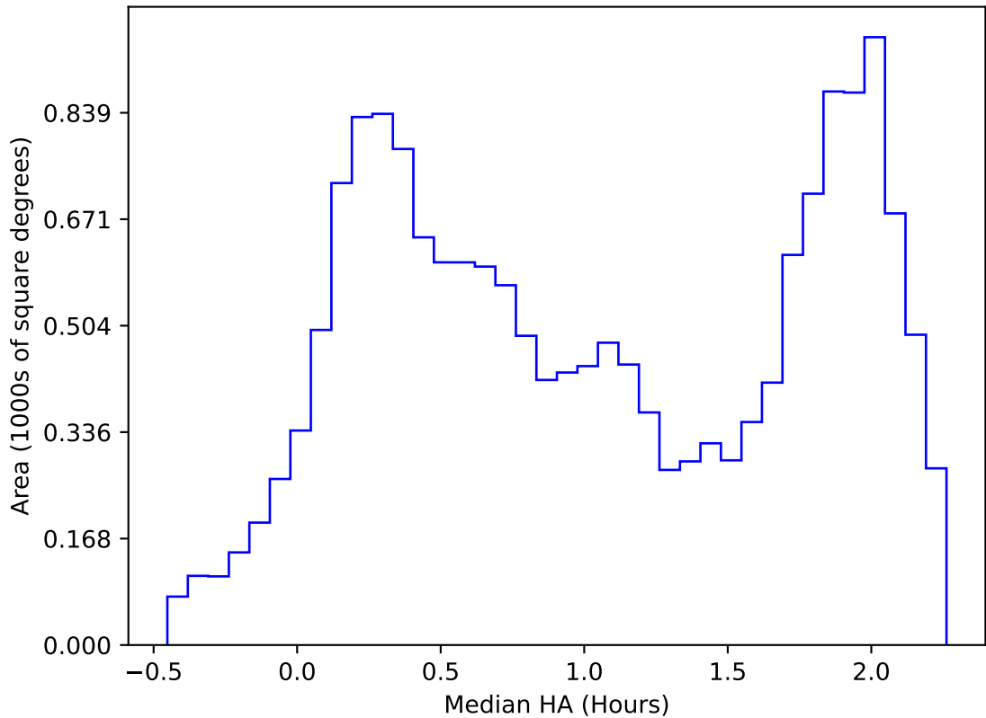
ddf_acor_sf20_lsf40_lsr50_v3.4_10yrs WFD i band: Median HA
