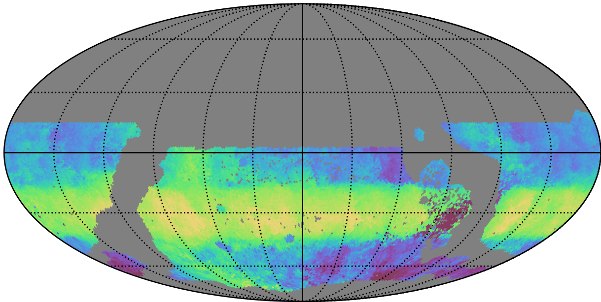
ddf_acor_sf20_lsf40_lsr50_v3.4_10yrs WFD g band: Median HA
