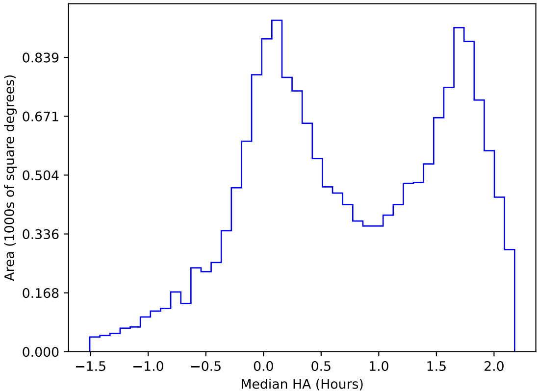
ddf_acor_sf20_lsf40_lsr50_v3.4_10yrs WFD g band: Median HA
