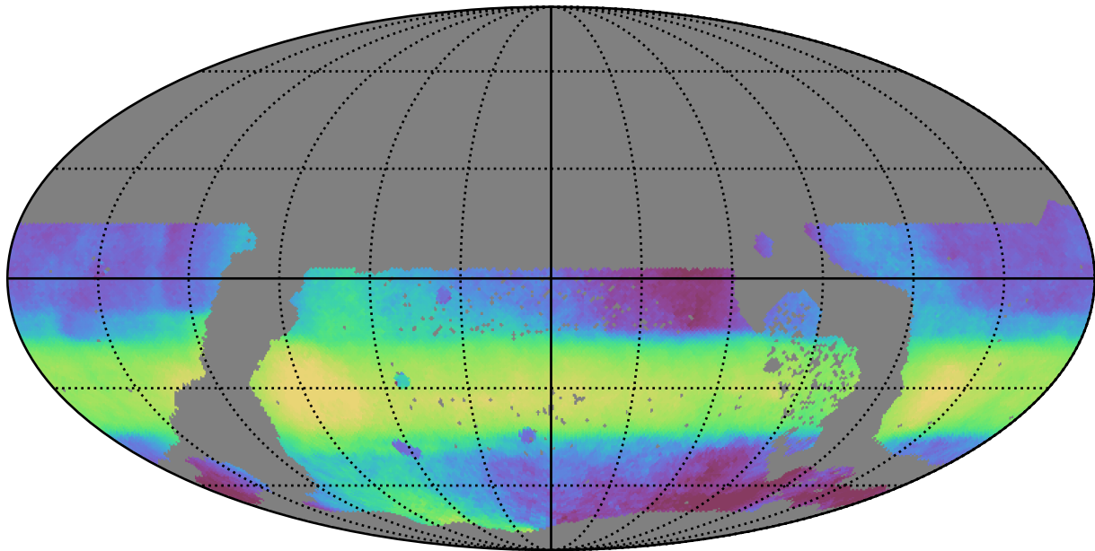
ddf_acor_sf20_lsf40_lsr50_v3.4_10yrs WFD all bands: Median HA
