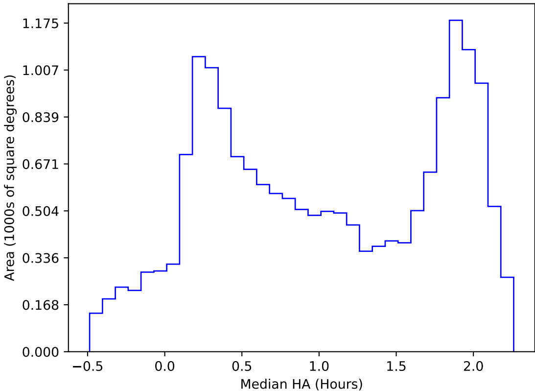
ddf_acor_sf20_lsf40_lsr50_v3.4_10yrs WFD all bands: Median HA
