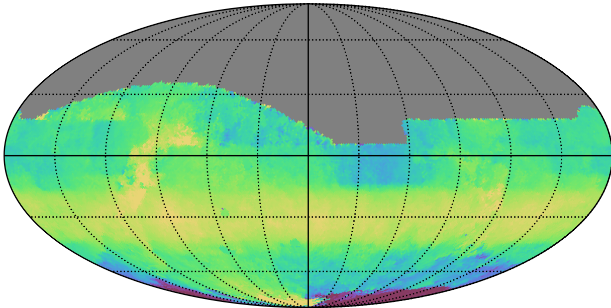
ddf_acor_sf20_lsf40_lsr50_v3.4_10yrs All sky z band: Median HA
