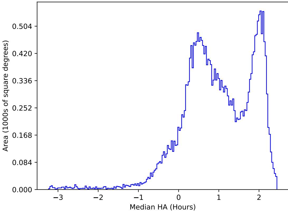
ddf_acor_sf20_lsf40_lsr50_v3.4_10yrs All sky z band: Median HA
