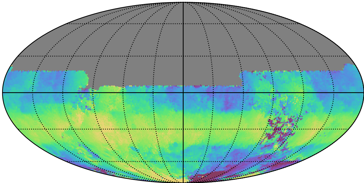
ddf_acor_sf20_lsf40_lsr50_v3.4_10yrs All sky u band: Median HA
