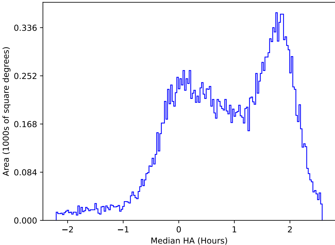
ddf_acor_sf20_lsf40_lsr50_v3.4_10yrs All sky u band: Median HA
