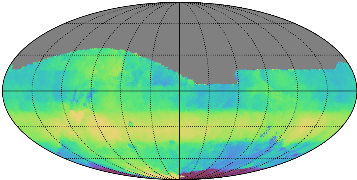
ddf_acor_sf20_lsf40_lsr50_v3.4_10yrs All sky r band: Median HA
