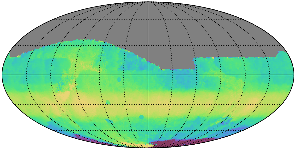
ddf_acor_sf20_lsf40_lsr50_v3.4_10yrs All sky i band: Median HA
