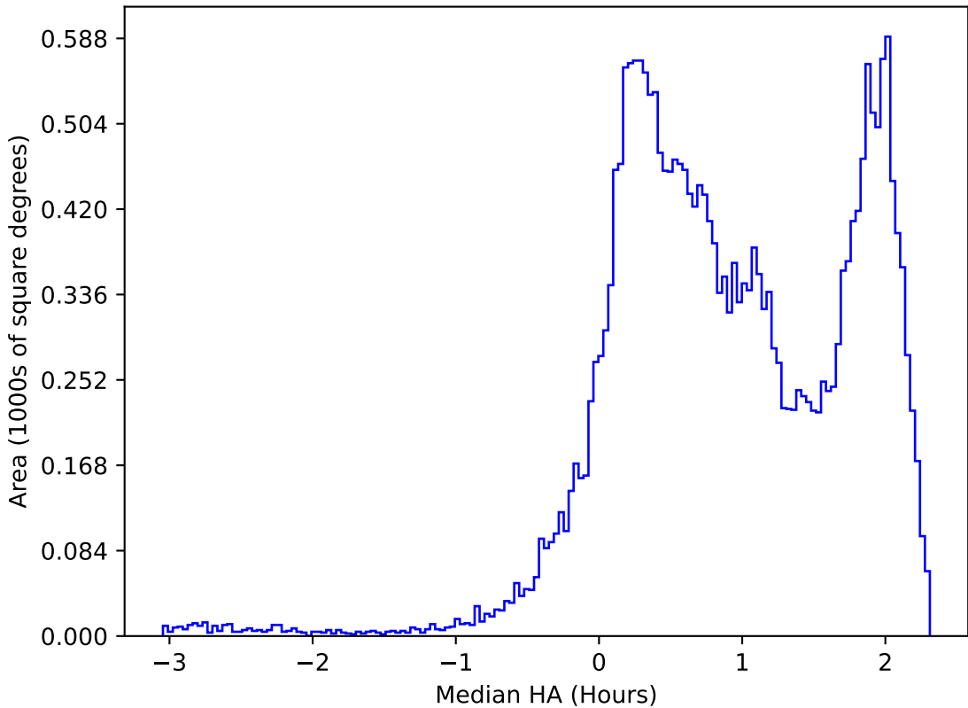
ddf_acor_sf20_lsf40_lsr50_v3.4_10yrs All sky i band: Median HA
