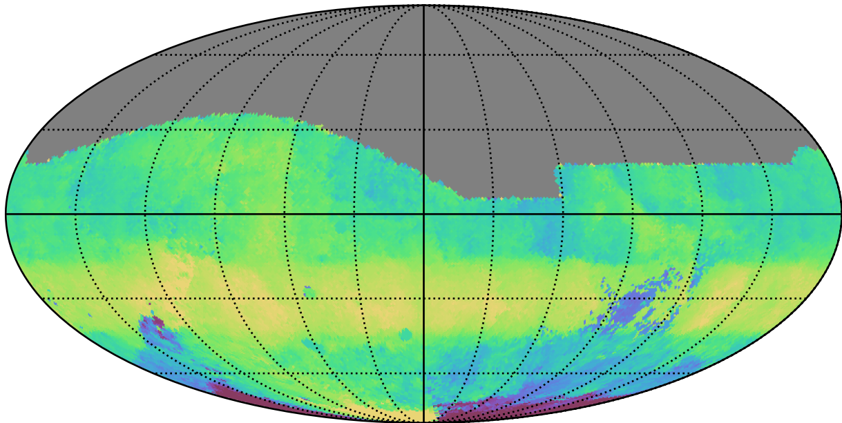
ddf_acor_sf20_lsf40_lsr50_v3.4_10yrs All sky g band: Median HA
