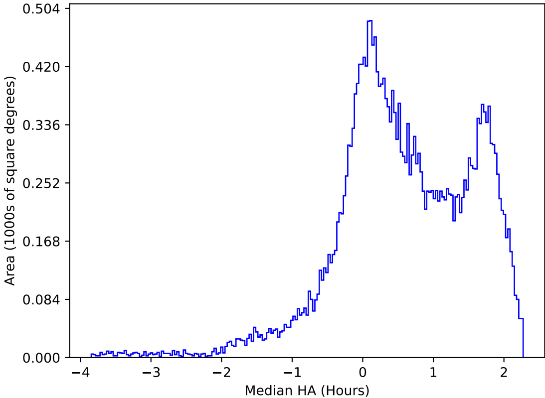
ddf_acor_sf20_lsf40_lsr50_v3.4_10yrs All sky g band: Median HA
