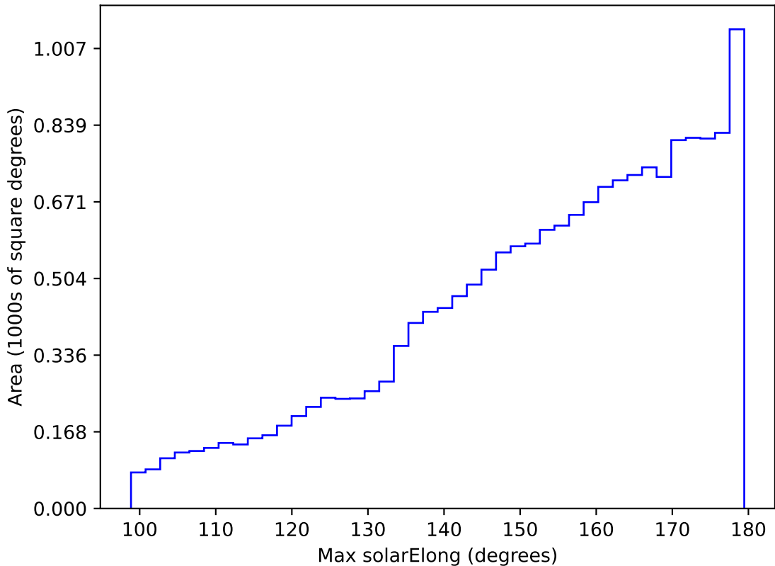
ddf_acor_sf20_lsf40_lsr50_v3.4_10yrs WFD z band: Max solarElong
