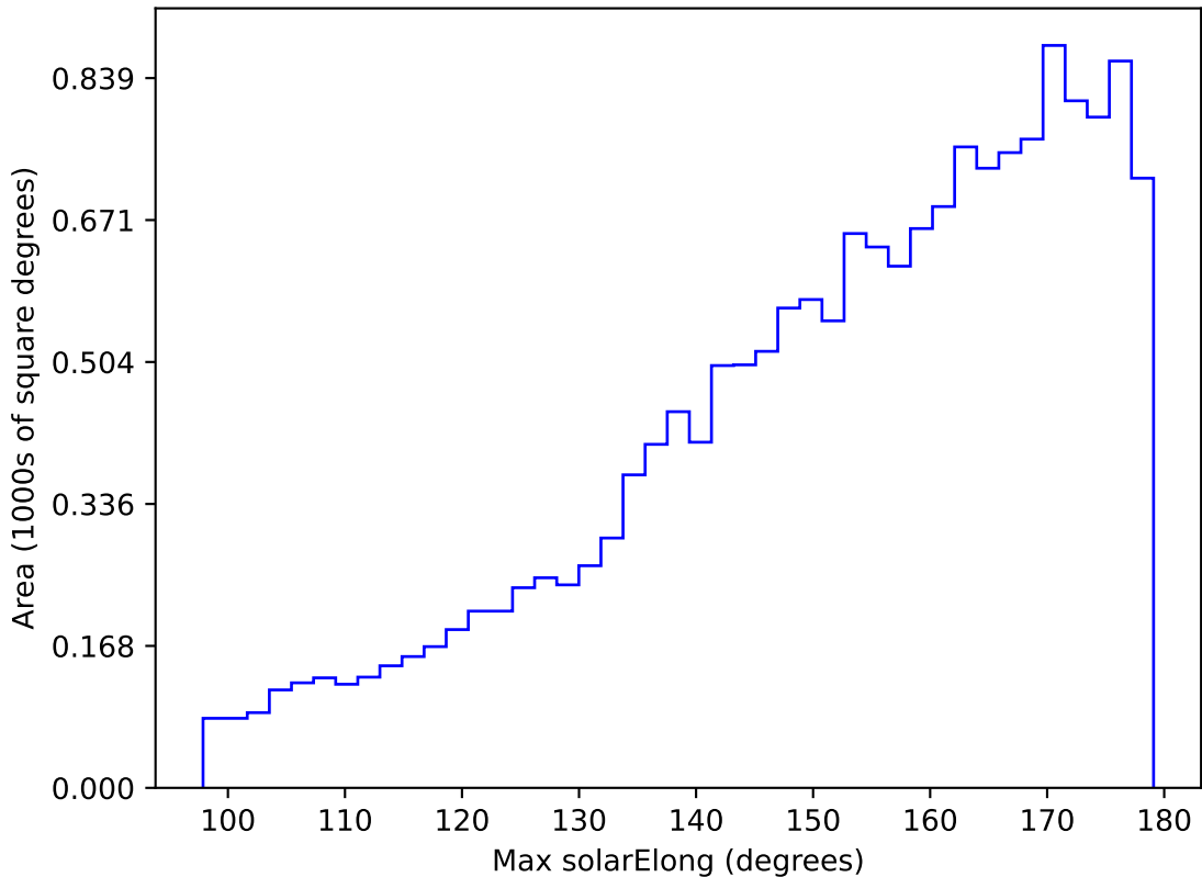
ddf_acor_sf20_lsf40_lsr50_v3.4_10yrs WFD u band: Max solarElong
