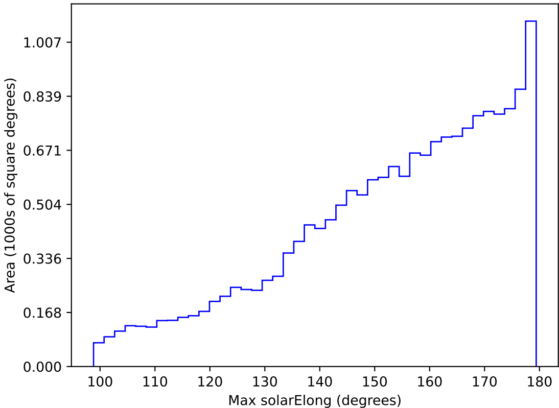
ddf_acor_sf20_lsf40_lsr50_v3.4_10yrs WFD r band: Max solarElong
