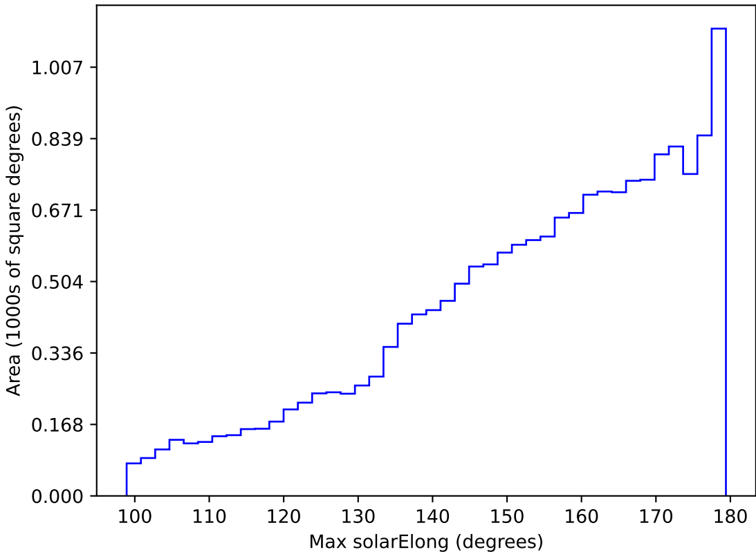
ddf_acor_sf20_lsf40_lsr50_v3.4_10yrs WFD i band: Max solarElong
