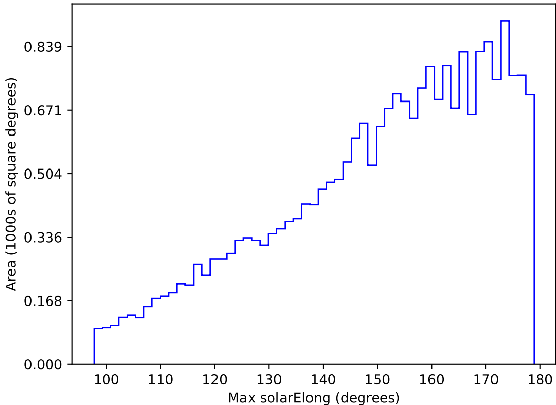
ddf_acor_sf20_lsf40_lsr50_v3.4_10yrs All sky u band: Max solarElong
