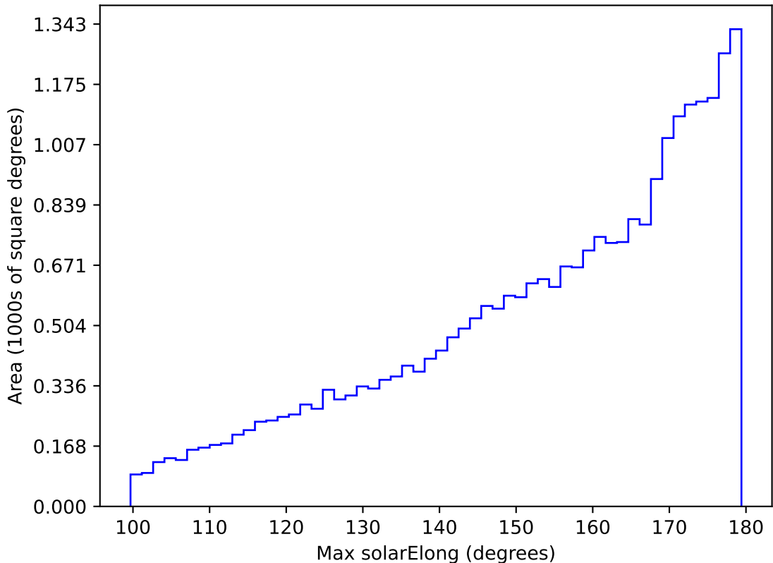
ddf_acor_sf20_lsf40_lsr50_v3.4_10yrs All sky r band: Max solarElong
