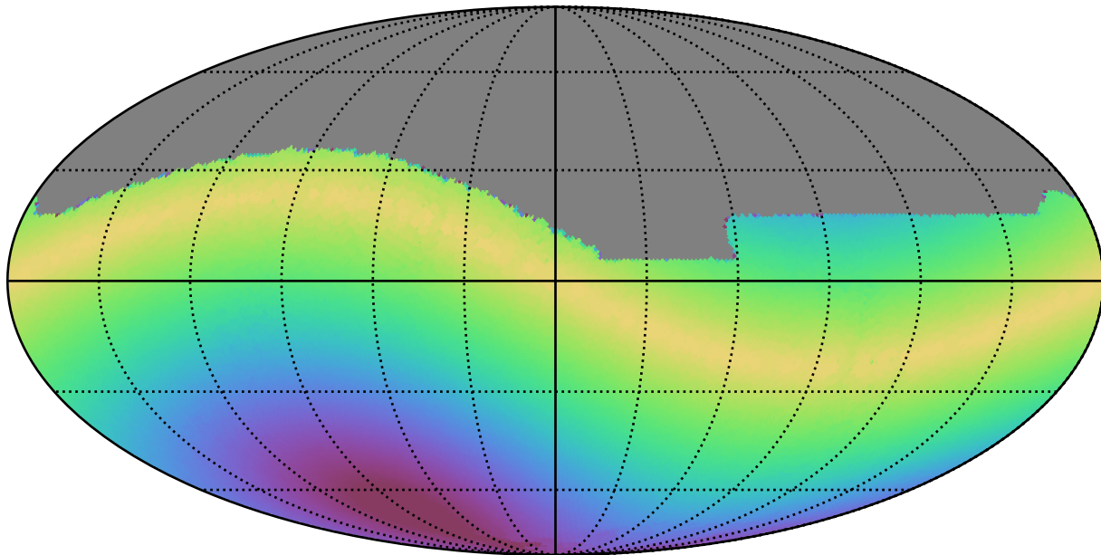
ddf_acor_sf20_lsf40_lsr50_v3.4_10yrs All sky i band: Max solarElong
