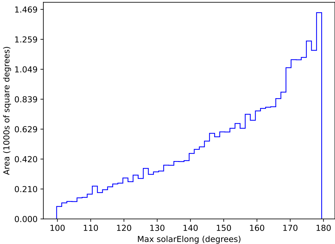
ddf_acor_sf20_lsf40_lsr50_v3.4_10yrs All sky i band: Max solarElong
