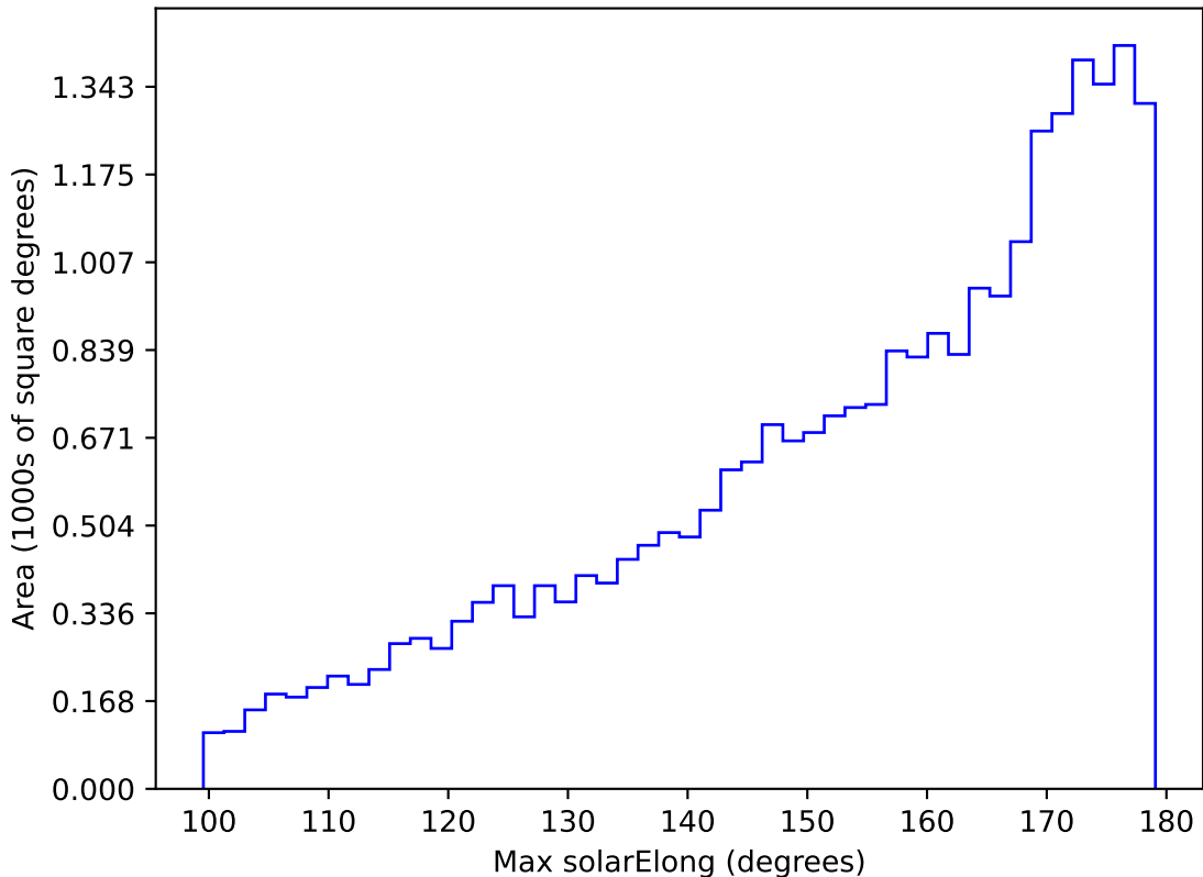
ddf_acor_sf20_lsf40_lsr50_v3.4_10yrs All sky g band: Max solarElong
