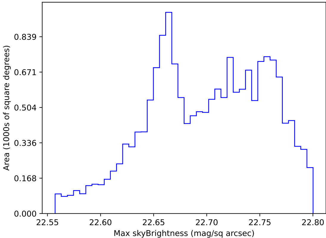
ddf_acor_sf20_lsf40_lsr50_v3.4_10yrs WFD u band: Max skyBrightness
