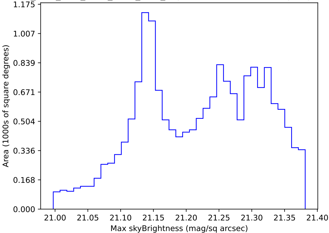
ddf_acor_sf20_lsf40_lsr50_v3.4_10yrs WFD r band: Max skyBrightness
