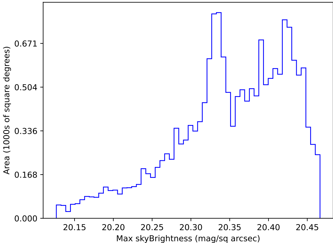
ddf_acor_sf20_lsf40_lsr50_v3.4_10yrs WFD i band: Max skyBrightness
