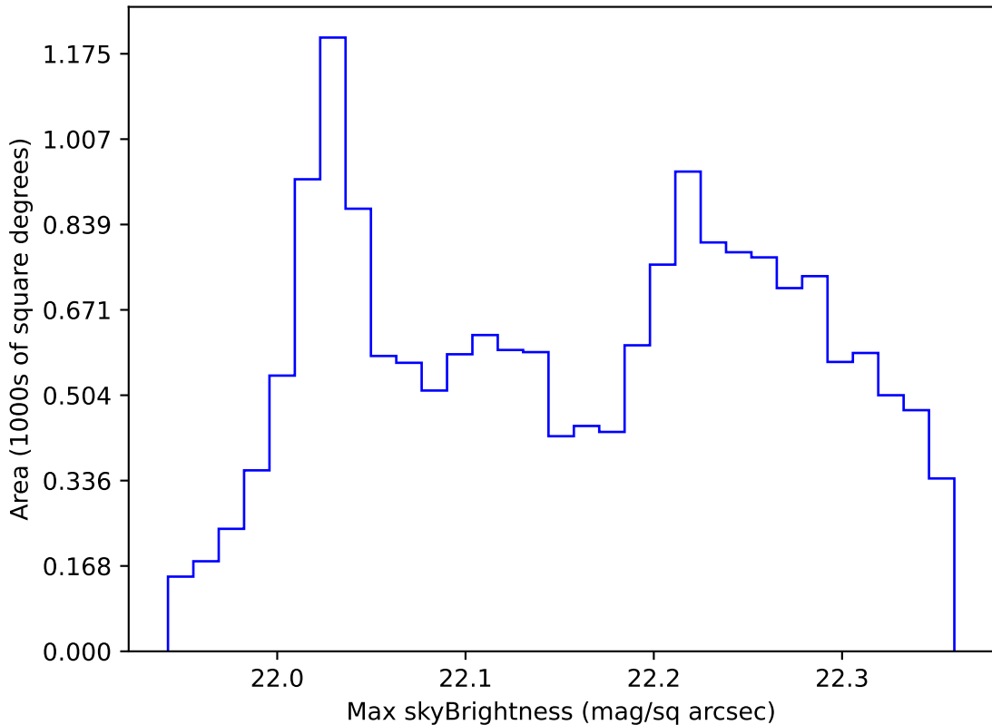
ddf_acor_sf20_lsf40_lsr50_v3.4_10yrs WFD g band: Max skyBrightness
