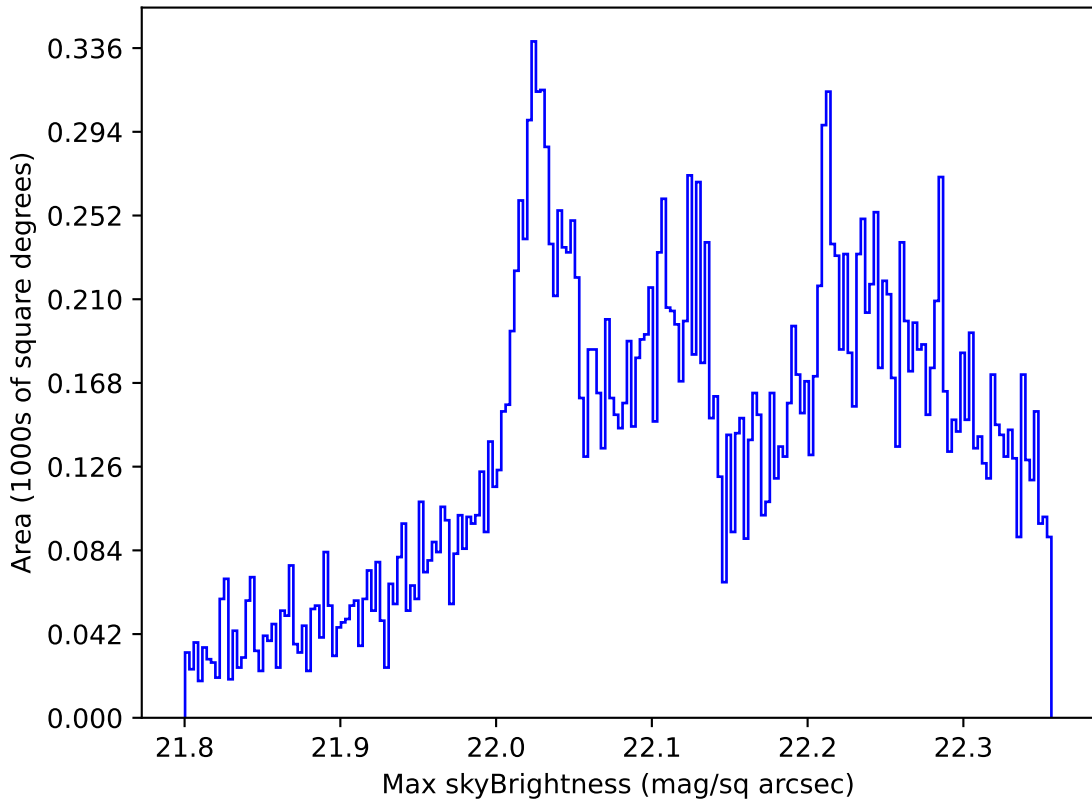
ddf_acor_sf20_lsf40_lsr50_v3.4_10yrs All sky g band: Max skyBrightness
