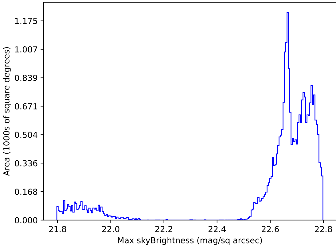
ddf_acor_sf20_lsf40_lsr50_v3.4_10yrs All sky all bands: Max skyBrightness
