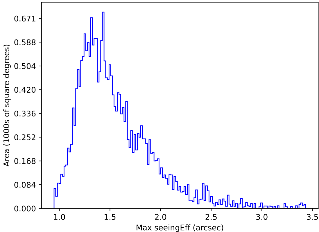
ddf_acor_sf20_lsf40_lsr50_v3.4_10yrs Yr 1 u band: Max seeingEff
