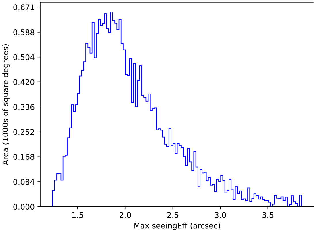
ddf_acor_sf20_lsf40_lsr50_v3.4_10yrs Yr 1 all bands: Max seeingEff
