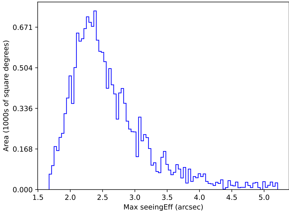
ddf_acor_sf20_lsf40_lsr50_v3.4_10yrs WFD z band: Max seeingEff
